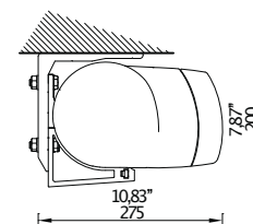
Ceiling installation
